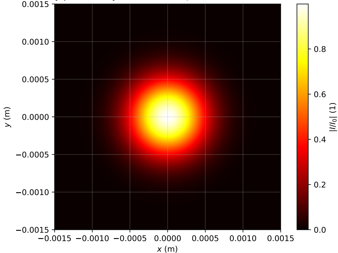
Intensity profile I(x, y, z = 0.080m)/I_0 , P_{in}=0.1P_{cr} , artificial time
